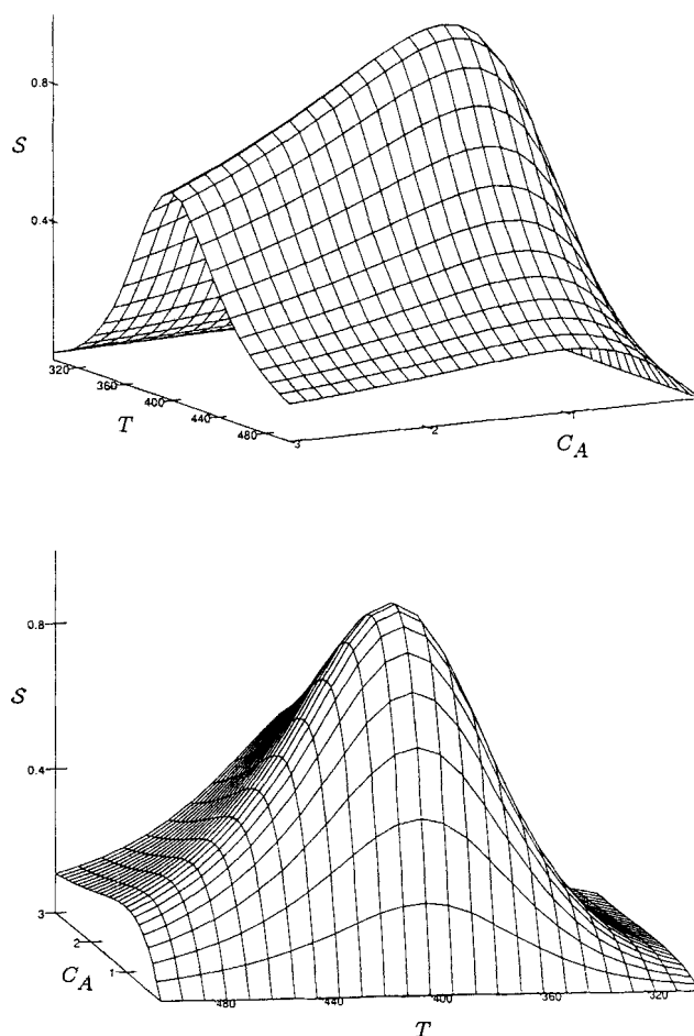
Figure 3. Reaction selectivity vs. C_A and T , at steady-state conditions.
